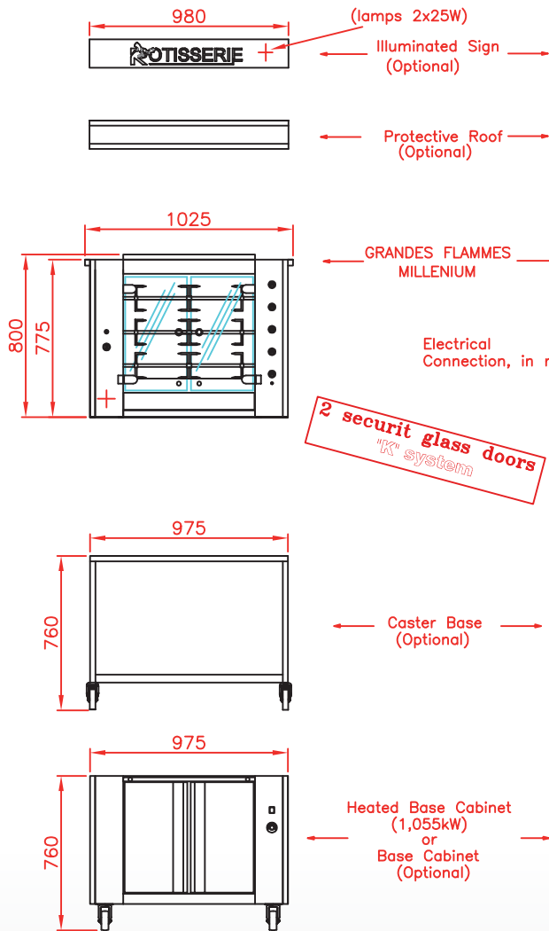
Front view Rotisserie with roof (optional) and base on casters (optional)
