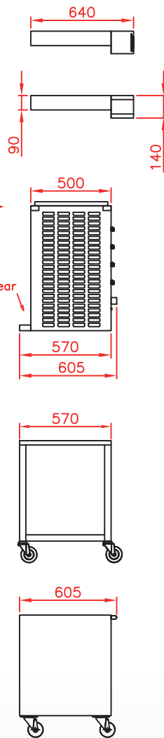
Side view Rotisserie with roof (optional) and base on casters (optional)
